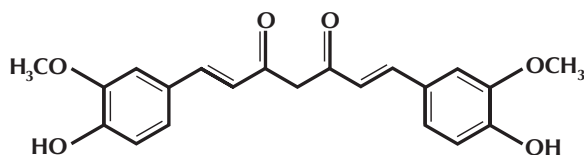
Figure 2: Molecular Structure of Curcumin
